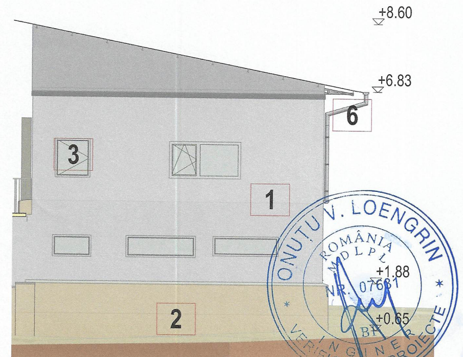
FATADA LATERAL STANGA
