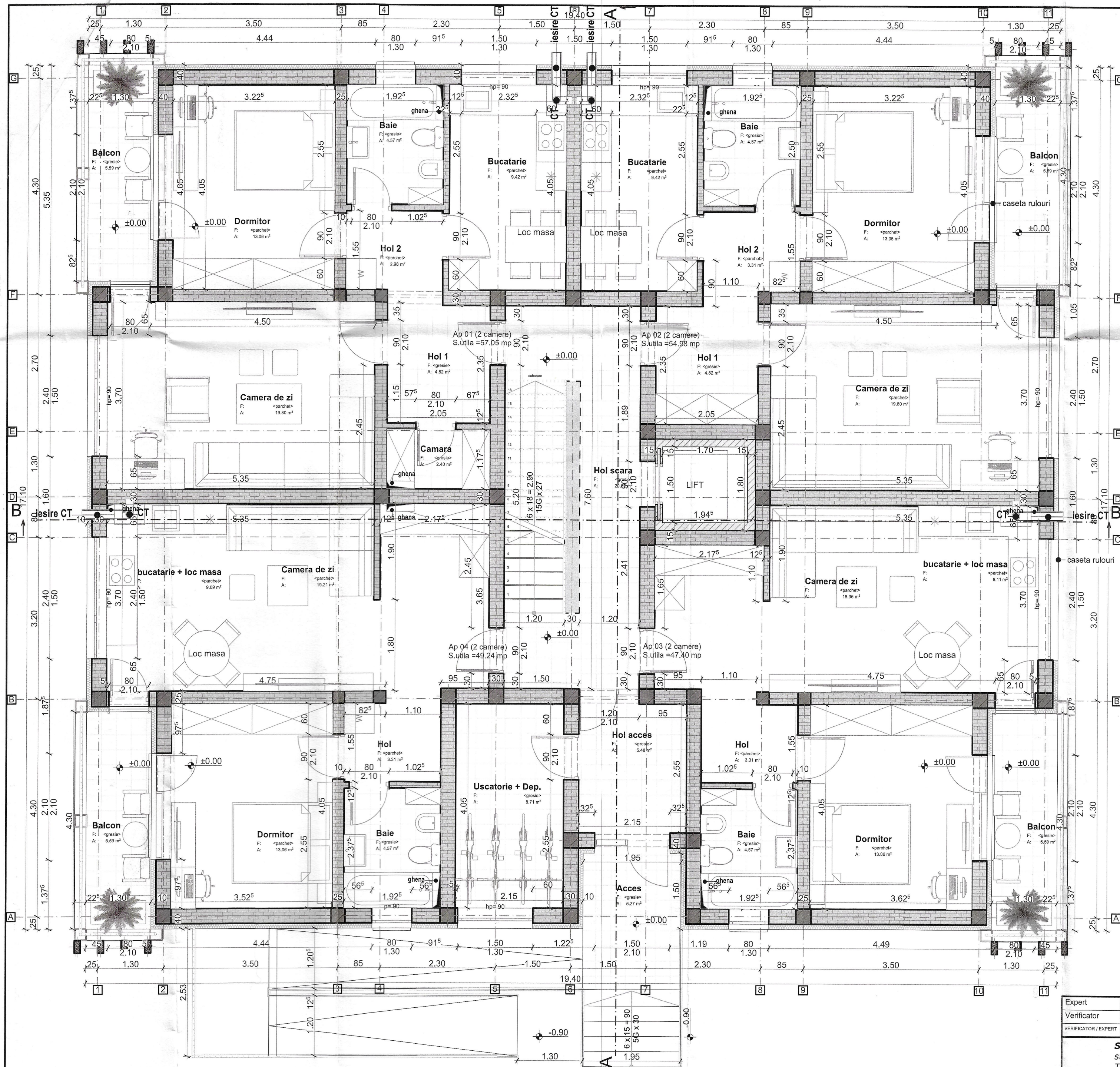
PLAN PARTER scara 1:50
