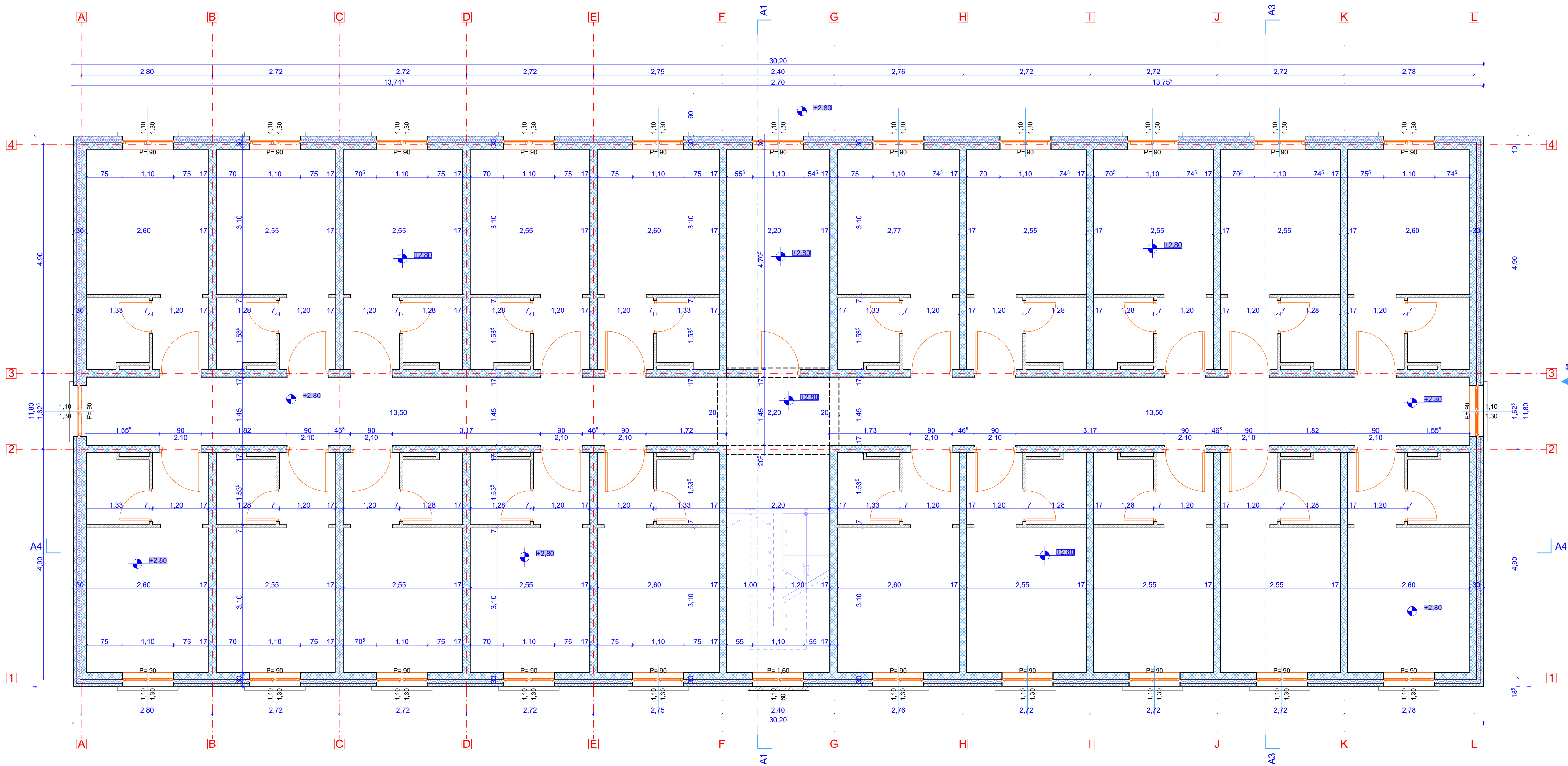
PLAN ETAJ 1-RELEVU (cota + 2.80m)
