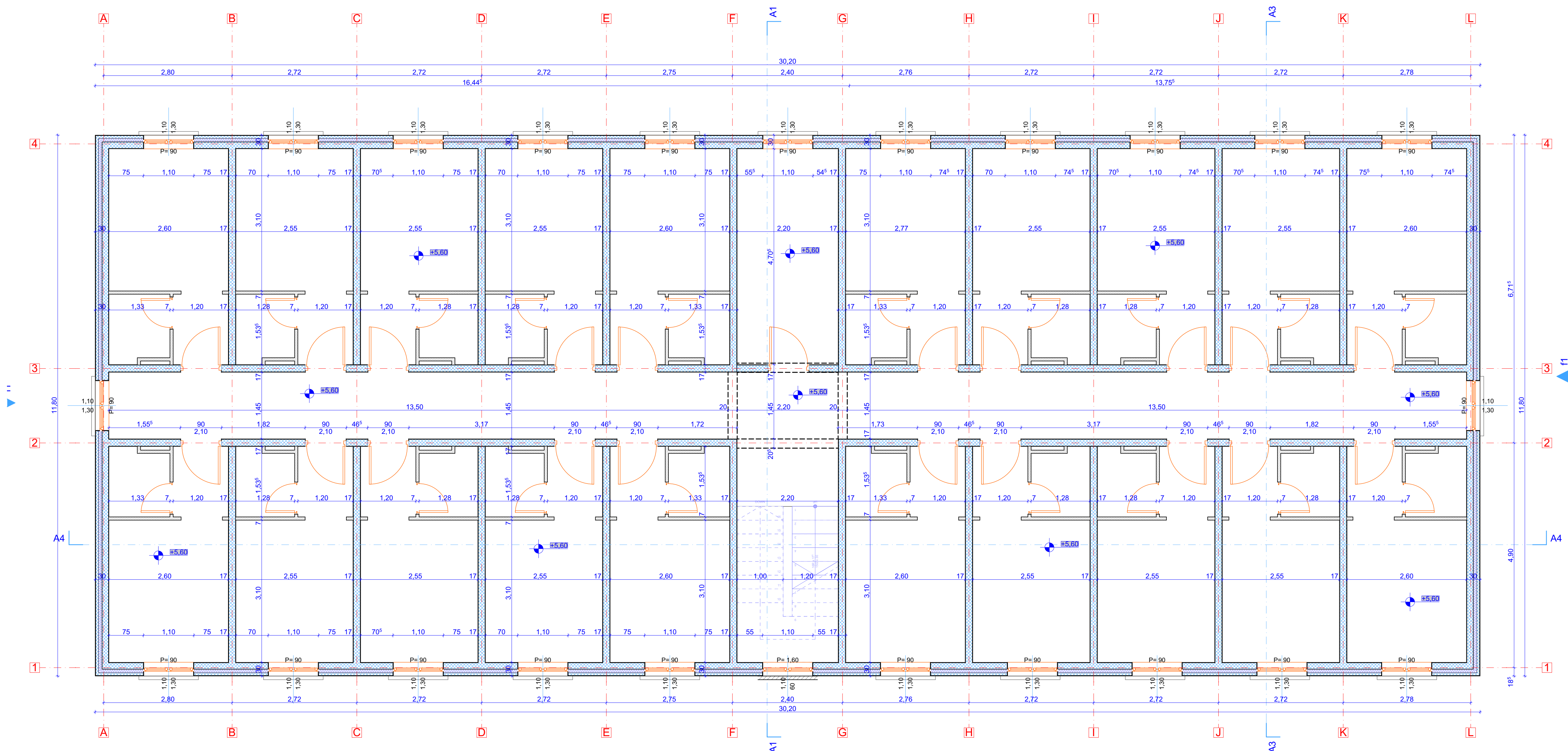
PLAN ETAJ 2-RELEVU (cota + 5.60m)
