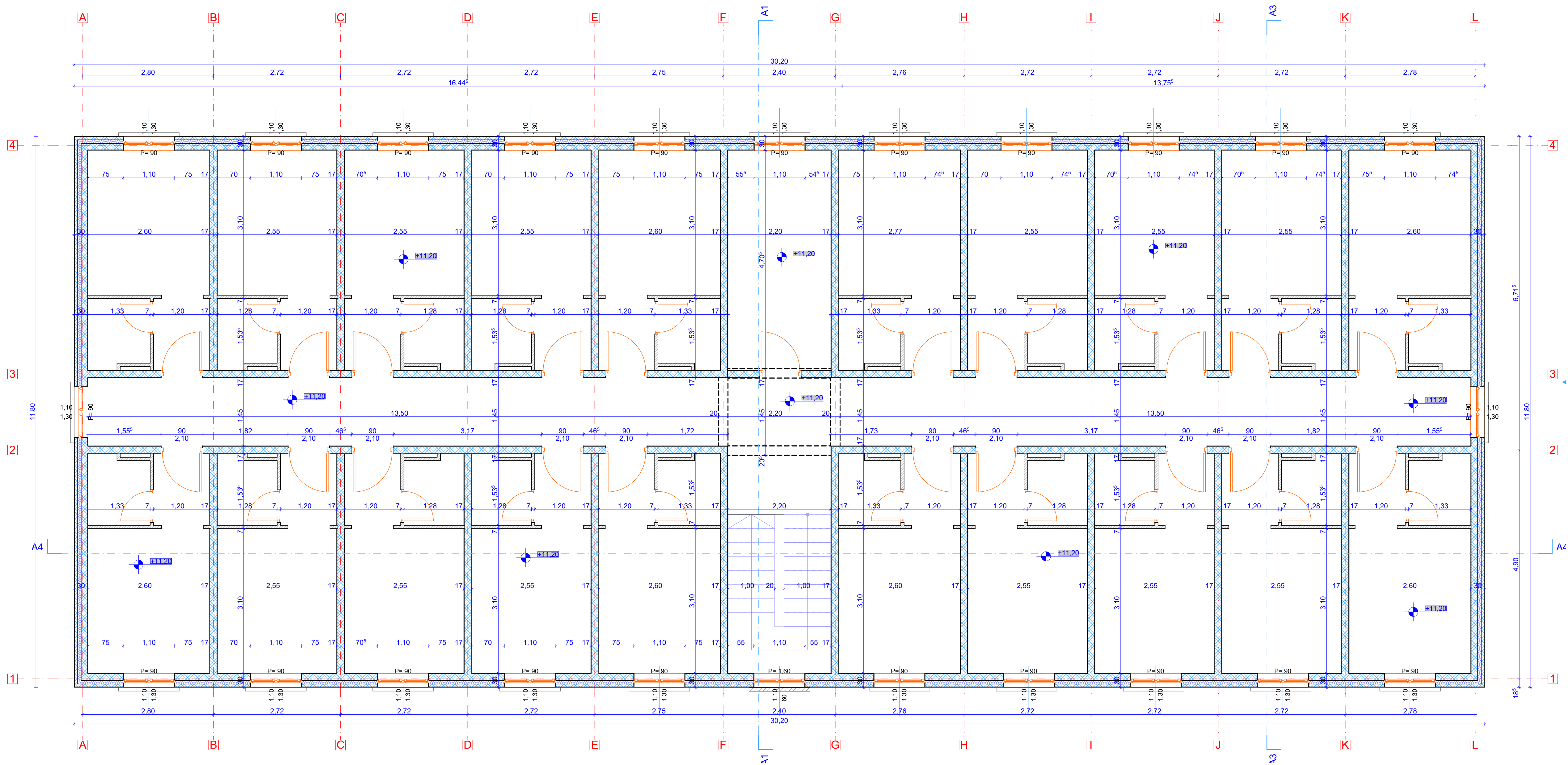
PLAN ET AJ 4-RELEVU (cota + 11.20m)
