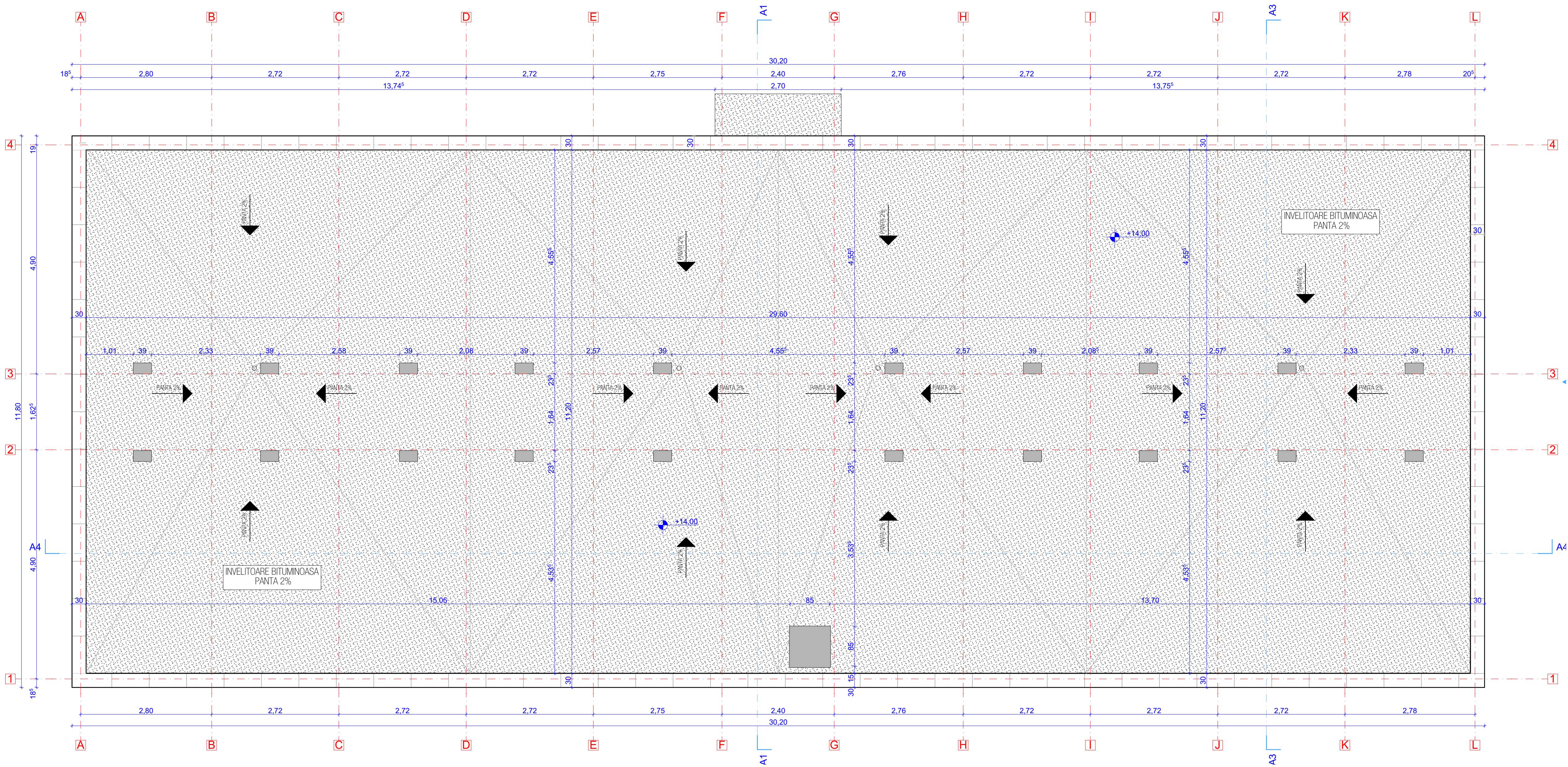
PLAN INVELITOARE-RELEVU
