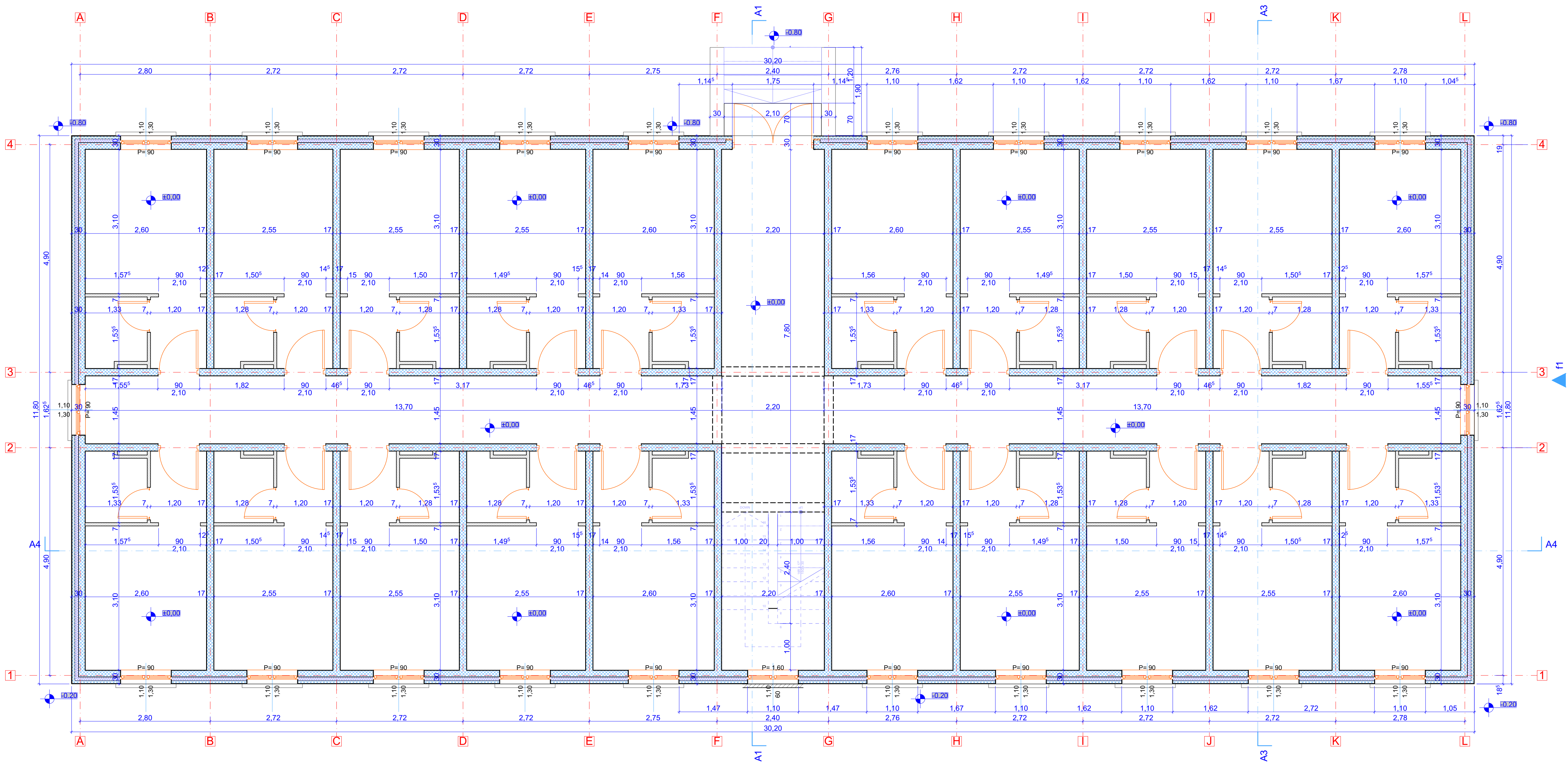
PLAN PARTER-RELEVU (cota ± 0.00m)
