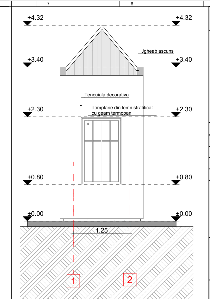
FATADA VEST
