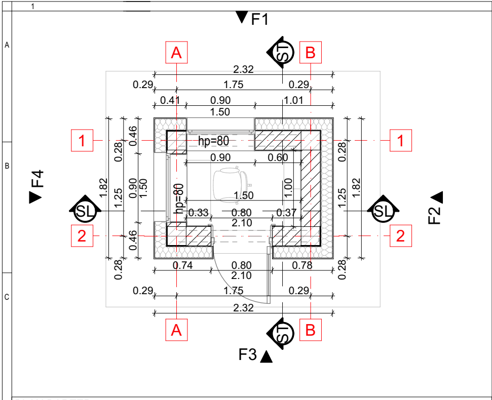
PLAN PARTER
