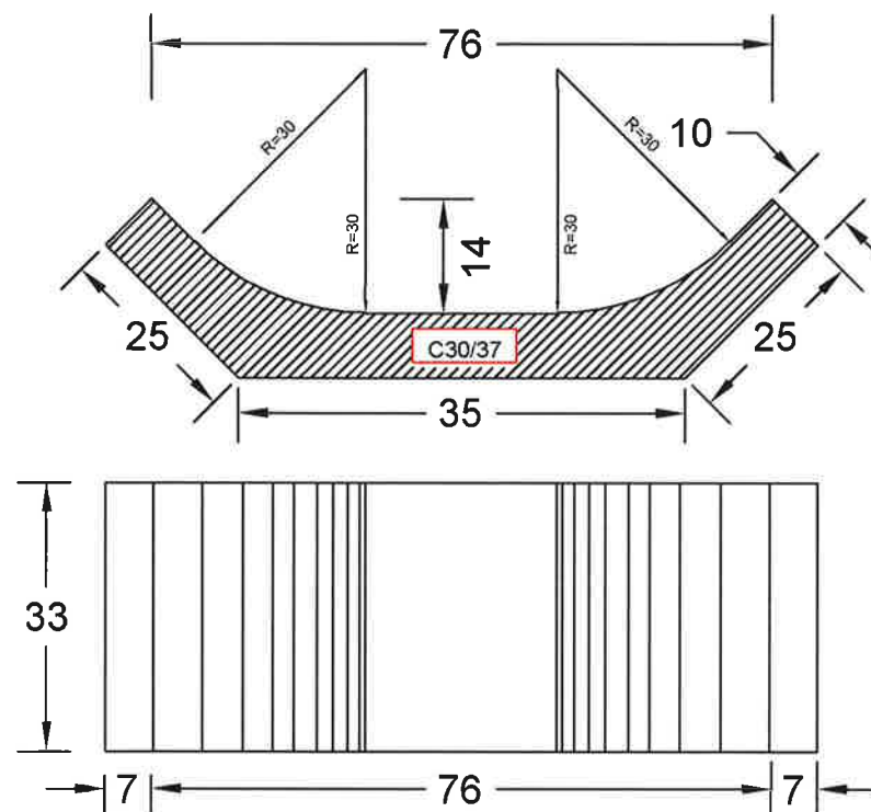
ELEMENT MONOLIT TIP 1 40 x 33 x 10
