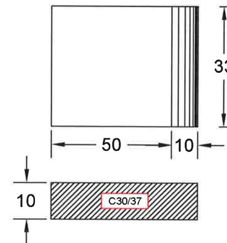
ELEMENT MONOLIT TIP 2 60 x 33 x 10
