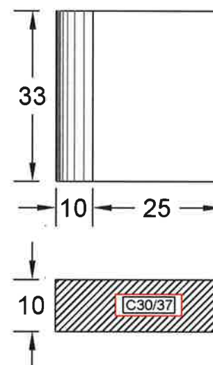
ELEMENT MONOLIT TIP 4 35 x 33 x 10
