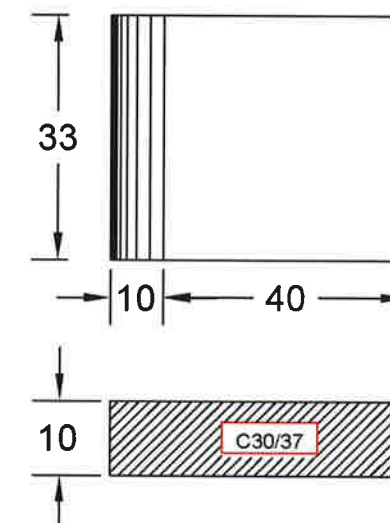
ELEMENT MONOLIT TIP 3 35 x 33 x 10
