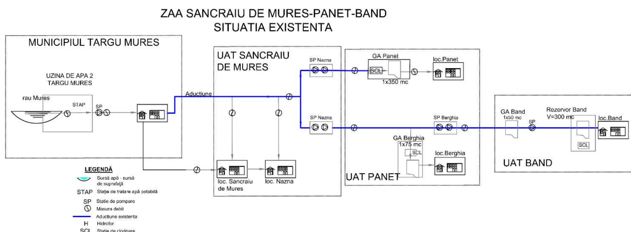
Figura Error! No text of specified style in document. -33 – Schema sistem de apa potabila din ZAA Targu Mures – Panet - Band
