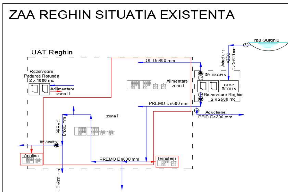
Figura Error! No text of specified style in document. -38 – Schema conductelor de transport apa potabila din ZAA Reghin
